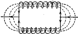
FIG. 2. — THE BINOCULAR TYPE OF WINDING DISCUSSED IN THE TEXT The magnetic field threads through both coils and there is little external field. Because two coils are in parallel, each will have to be larger than a single coil if it were employed.
