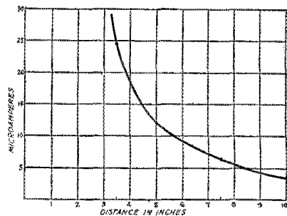
FIG. 4.— This curve is for a high-vacuum cell and shows the relationship between the current output of the cell and the distance between the cell and the source of illumination which is approximately equivalent to a 300-watt Mazda lamp operated at 115 volts.
