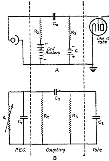
FIG. 6.— THE UPPER PORTION LABELLED A GIVES THE SCHEMATIC DIAGRAM OF THE COUPLING BETWEEN THE CELL AND THE GRID OF THE TRIOD
