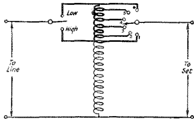
FIG. 1. — THE CIRCUIT ARRANGEMENT OF THE AUTO TRANSFORMER IS GIVEN ABOVE
